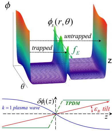
FIG. 1: (Color online) Top: \theta -symmetric end confinement and central separatrix potentials, modified by an \ell = 1 z -anti-symmetric error field, and an m = 2 ruffle on the separatrix. Bottom: z -dependence of 3 error fields considered here.
