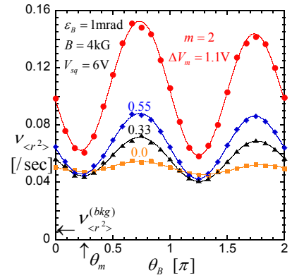
FIG. 2: (Color online) Measured expansion rate \nu_{\langle r^2 \rangle} , showing chaotic NCT varying as \sin^2(\theta_B - \theta_m) , and \alpha -independent collisional transport.
