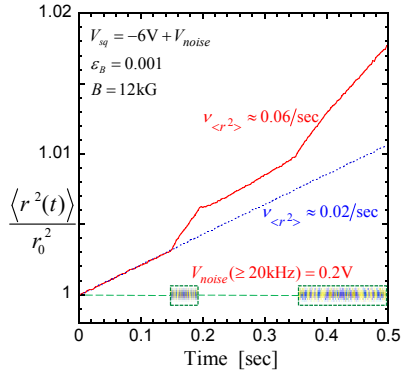
FIG. 4: (Color online) Enhanced expansion rate during two bursts of 200 mV (RMS) noise applied to a 6. V electrostatic separatrix.
