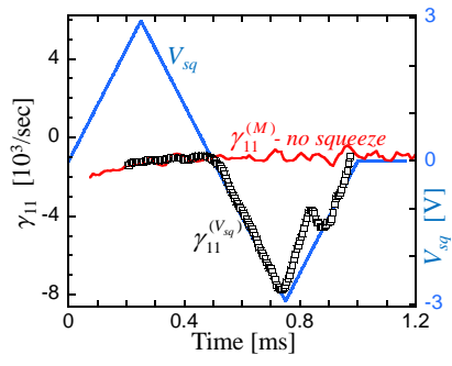
FIG. 6: (Color online) Separatrix damping of a Langmuir wave: \gamma_{11}^{(M)} from a weak magnetic mirror (red); and \gamma_{11}^{(V_{sq})} (black) due to a ramped \theta -symmetric negative V_{sq} (blue).
