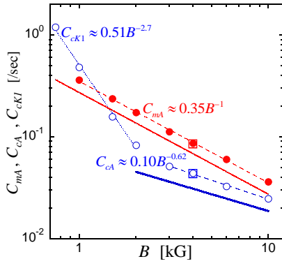
FIG. 3: (Color online) Measured transport rates C versus magnetic field B , with empirical scalings. Solid lines are the theory predictions.
