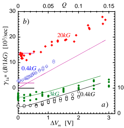
FIG. 5: (Color online) a) (bottom, right scales) TPDM damping rate \gamma_{1\alpha} times B versus applied m = 2 ruffle \Delta V_m for B = 0.4 and 3.0 kG. b) (top, left scales) damping versus amplitude Q of an excited m = 2 diocotron mode.
