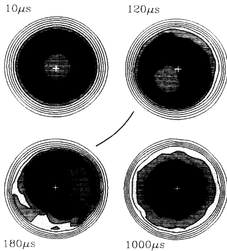
FIG. 2. Contour plots of the z -averaged density n(r, \theta) at four times during the l=1 instability. The contours are in increments of 0.6 \times 10^6 \text{ cm}^{-3} , and the highest four levels are shaded from gray to black.
