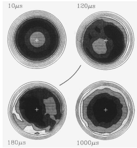
FIG. 2. Contour plots of the z -averaged density n(r, \theta) at four times during the l=1 instability. The contours are in increments of 0.6 \times 10^6 \text{ cm}^{-3} , and the highest four levels are shaded from gray to black.
