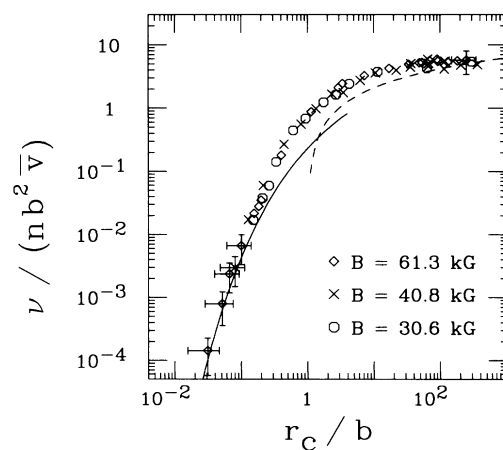
FIG. 4. Normalized rate vs r_c/b . For the \diamond , \times , and \circ data the magnetic fields are 61.3, 40.8, and 30.6 kG, respectively. For all the data \langle n \rangle = 8 \times 10^8 cm ^{-3} . The solid curve is the OH prediction. The dashed curve is the modified IR prediction.
